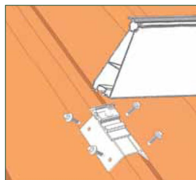
① Mounting of the Fix2000ClickTop connector.
