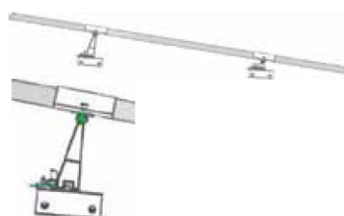
③ Mounting of the modules
