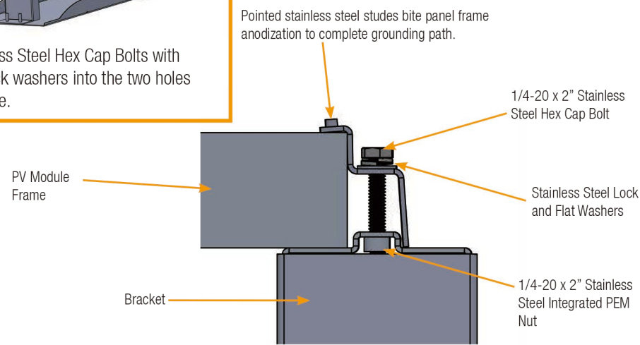
Detail View of Grounding End Plate
