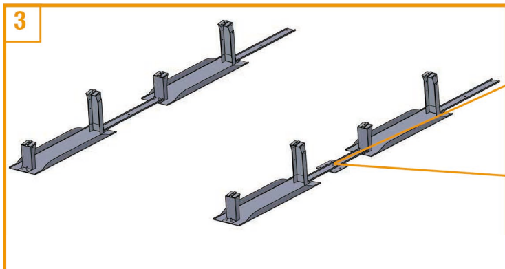
3 Add Connect Belts between each row over the top of the brackets on the PEM Studs. Add a 1/4-20 Stainless Steel Serrated Hex Flange Nut to each PEM Stud and tighten to 75 in-lb .
