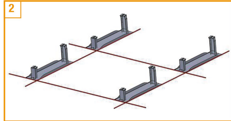
2 Place Brackets over integrated PEM Studs protruding out of each Ballast Pan (or Solar Belt). Do NOT secure hex flange nuts to PEM Studs at this time.
